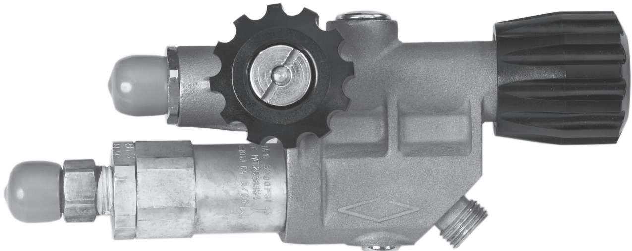
The properly assembled side block with the non-return valve and EGS adapter (inlet nipple) in position.
