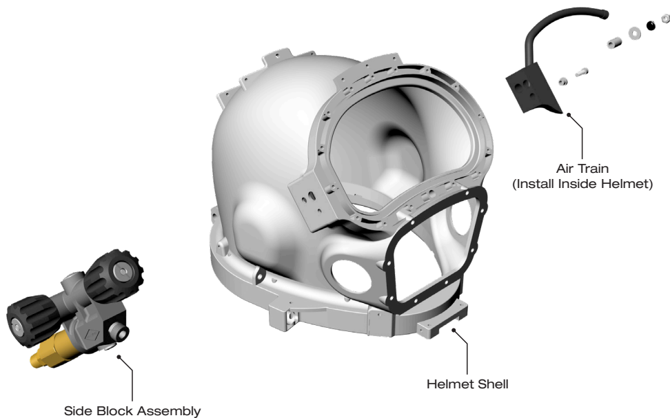
The fasteners that secure the side block also hold the air train in place.
