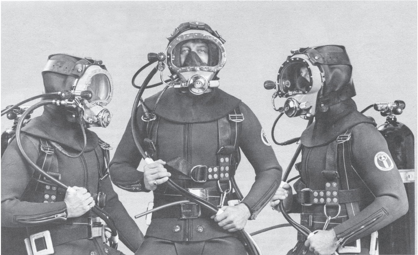
Diver wearing Model KMB-10 Band Mask with waterproof electrical connector and umbilical hose.
